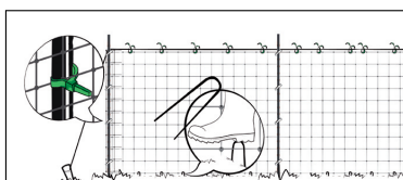
INSTALLATION WITH METAL T POST
