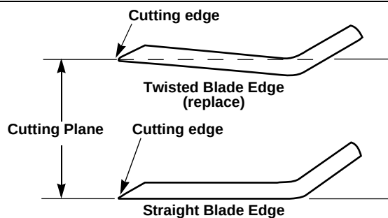
End view of blades, comparing twisted and straightened blades
