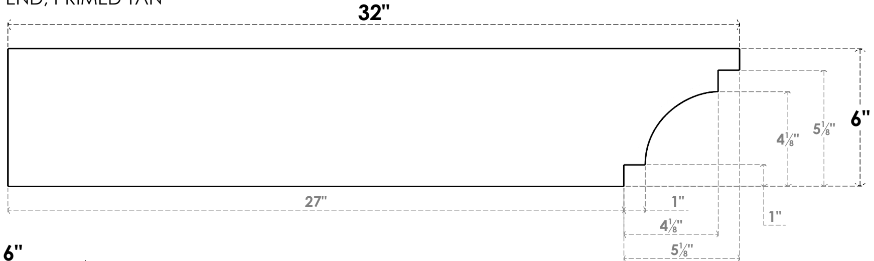
SIDE PROFILE
