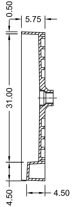
SECTION B-B
