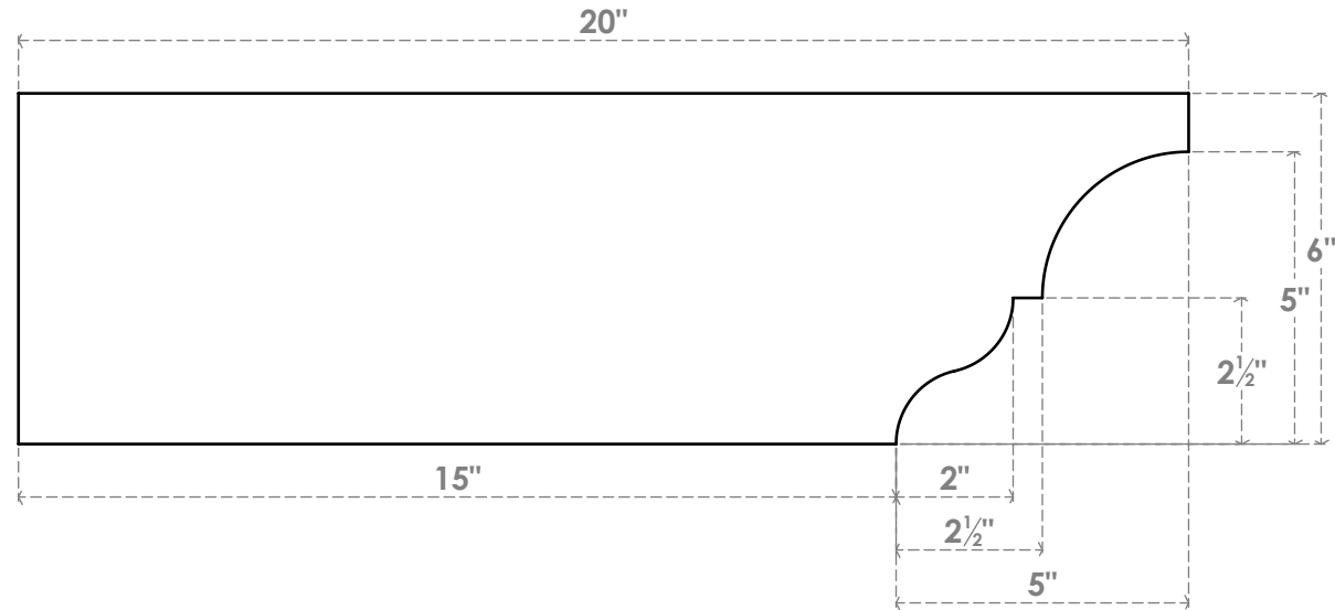
SIDE PROFILE
