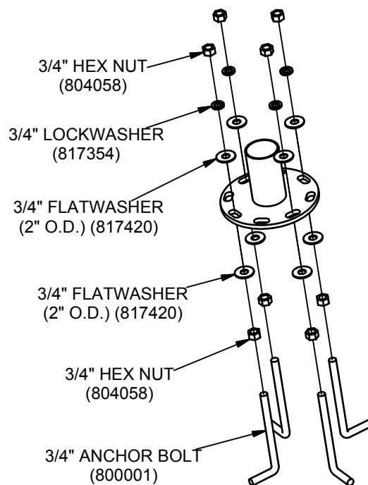
FOOTING ASSEMBLY DETAIL UP171F (FOOTING)
