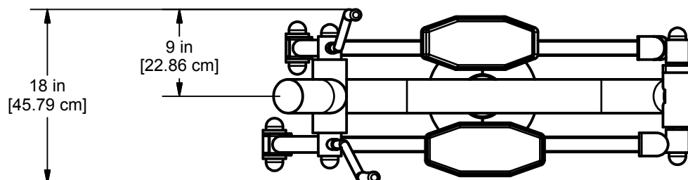
PLAN VIEW
