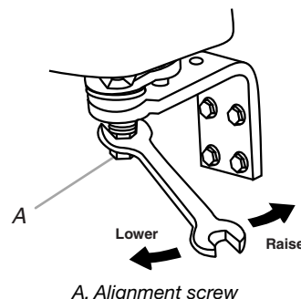
A. Alignment screw
