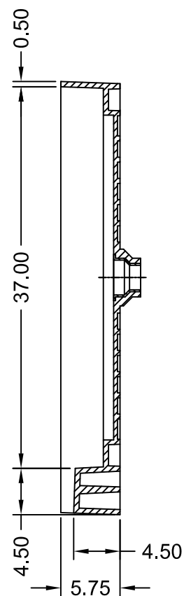
SECTION B-B
