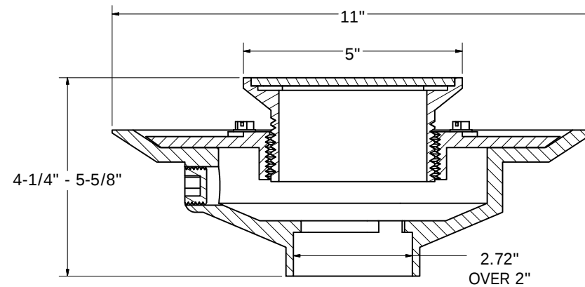
SECTION A-A SCALE .65
