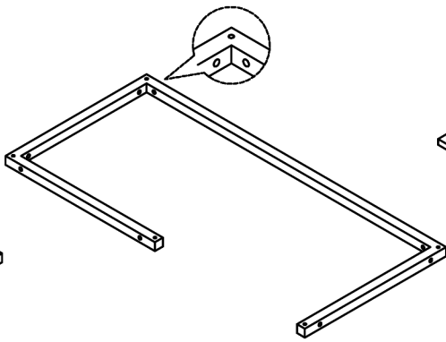
Bottom Frame
