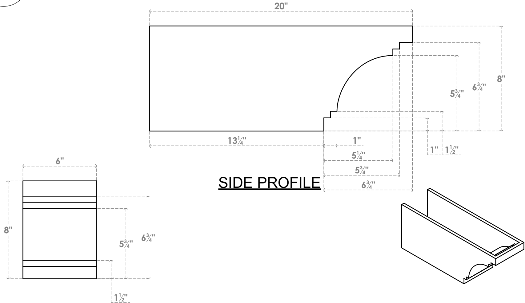
FRONT PROFILE
