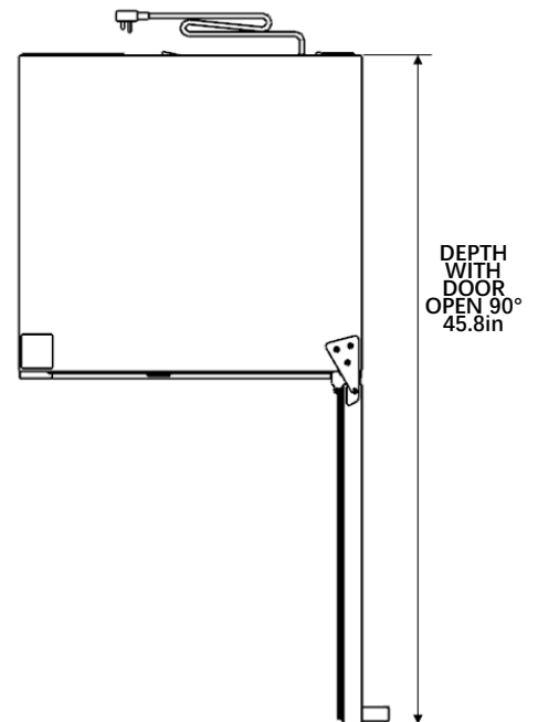
TOP OF BEVERAGE COOLER WITH DOOR OPEN 90°
