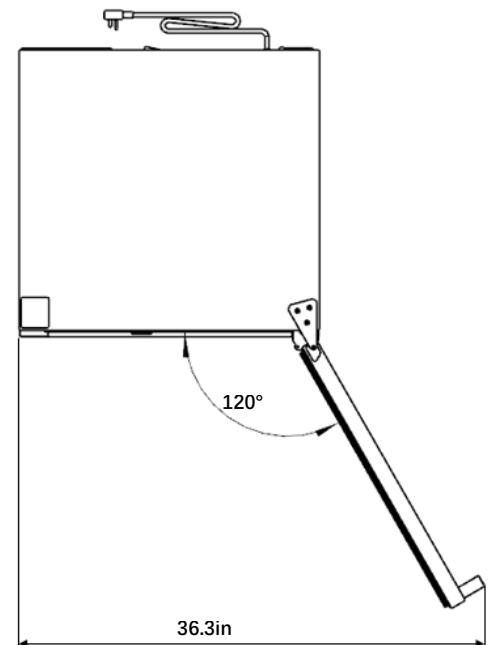
TOP OF BEVERAGE COOLER WITH DOOR OPEN 120 °
