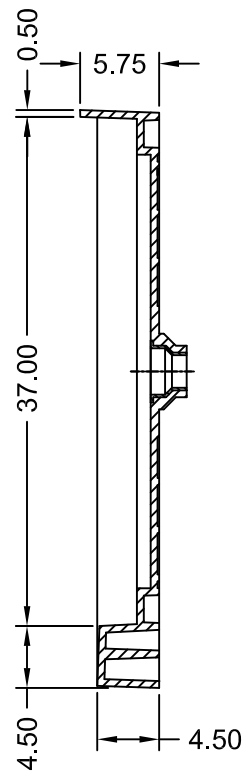
SECTION B-B
