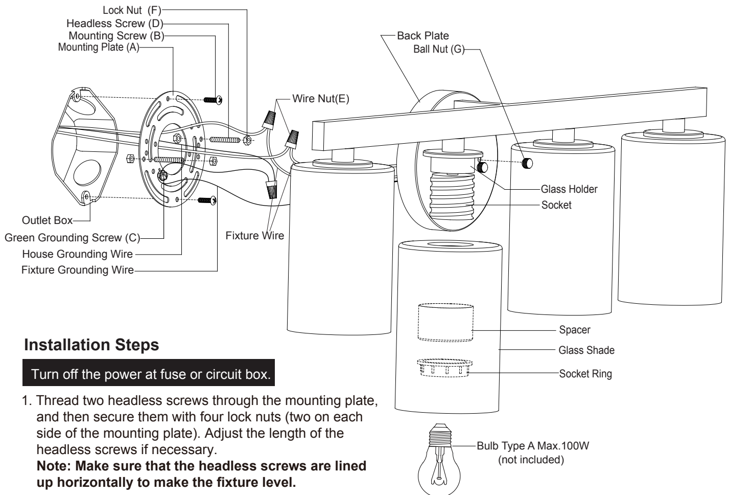
Green Grounding Screw (C)
