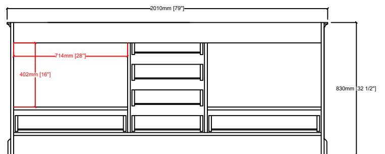
BACK VIEW
