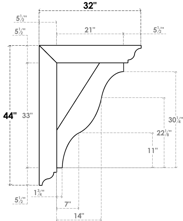
SIDE PROFILE
