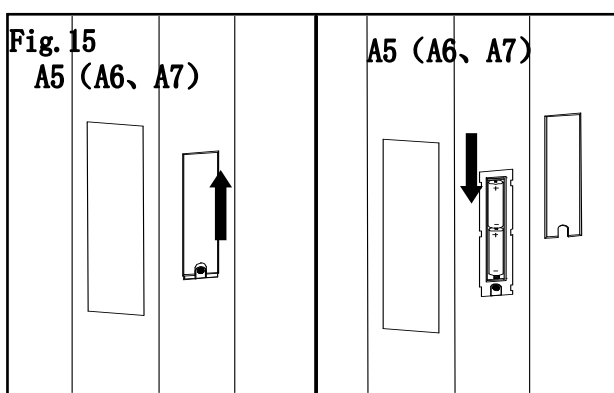
Fig.15: Remove battery holder cover, insert two (AA) battery, ( Note: to purchase "AA" battery ) then place cover on battery holder. Press the switch to control the light on and off.
