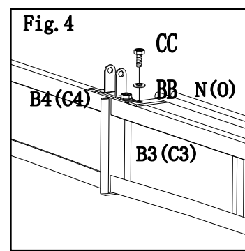
Fig.4: Attach mosquito netting rod (N、O) to across beam (B3、C3、B4、C4) by using bolt (CC) and flat washer (BB) ..
