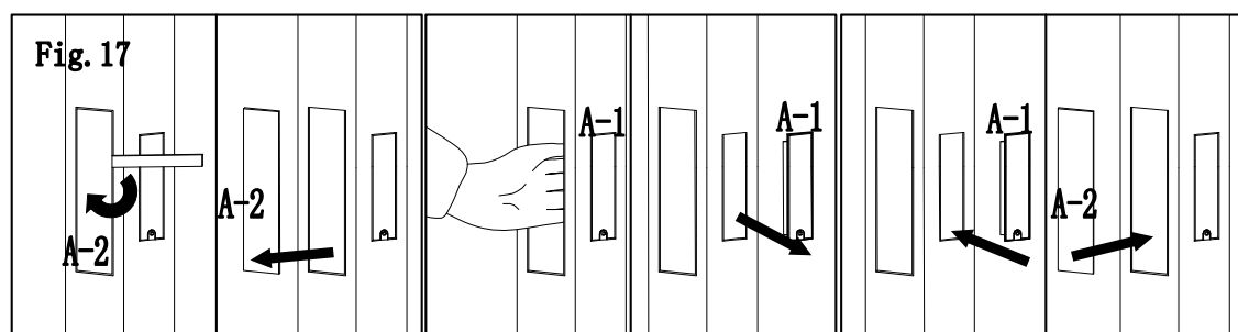
Fig.17: If the LED light or panel cover is old or damaged and need to be replaced, pry off the panel cover (A-2) along the gap between the panel and post with a thin film or simial tool, then replace the LED light (A-1) and put the panel cover on.
