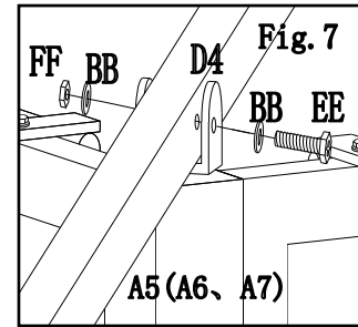
Fig.7: Fix sloping beam bottom tube (D4) to top of post (A5, A6, A7) by using bolt (EE) ,flat washer (BB) and nut (FF) .
