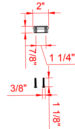
HANDLE
