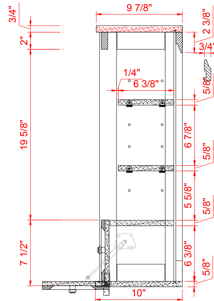
SIDE VIEW
