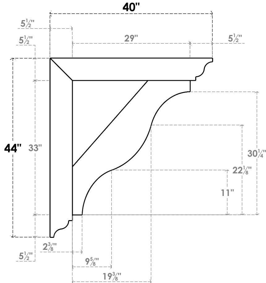
SIDE PROFILE
