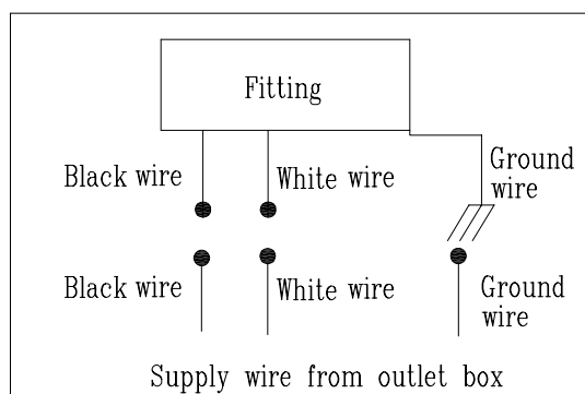
Circuit diagram 1
