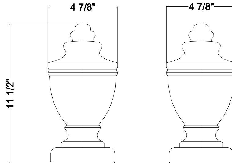
ITEM NUMBER:FIN04X11UR 4 7/8"OD x 11 1/2"H Urn Finial
