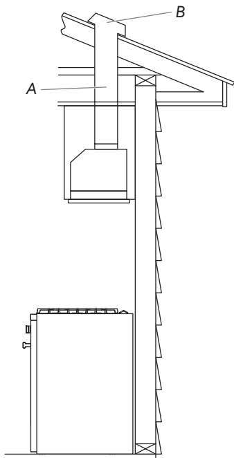
Roof Venting
