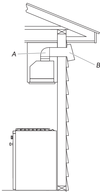
Wall Venting
