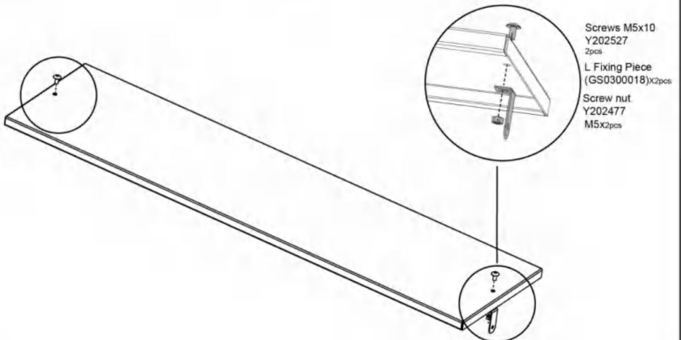
Shelf (GS0300009)X2pcs
