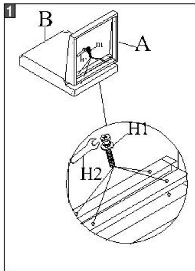
Step 1: Assemble seat cushion (B) with chair back (A).Using L-wrench (H2) to lock with 4*bolts (H1).
