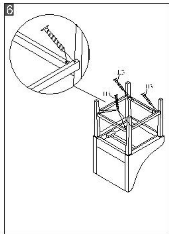
Step 6: Lock the stretchers tight with legs by using 8*screws (H3).
