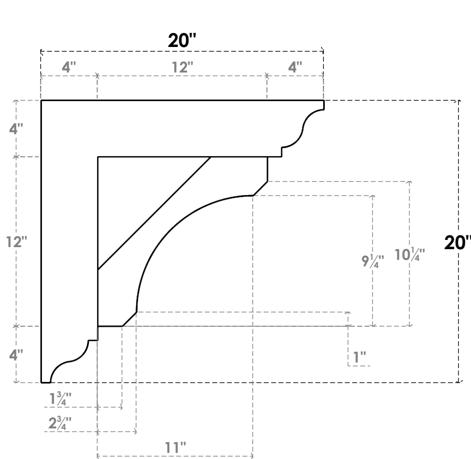
SIDE PROFILE
