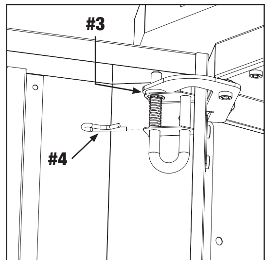
COTTER PIN ASSEMBLY
