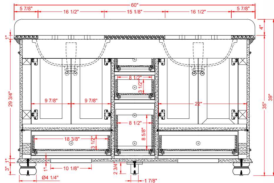
BACK VIEW
