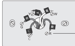
Terminal designation
