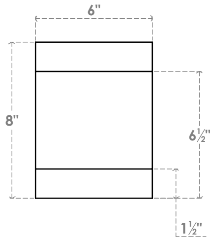
FRONT PROFILE
