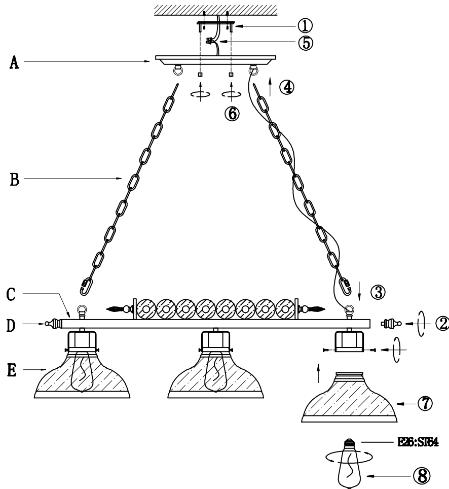
Installation sequence diagram
