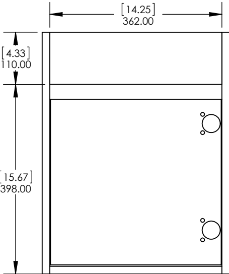
Back View / Vista Trasera
