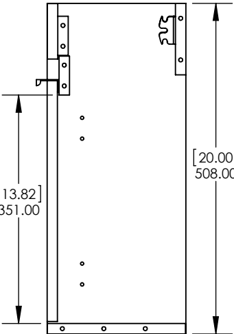
Side View / Vista Lateral
