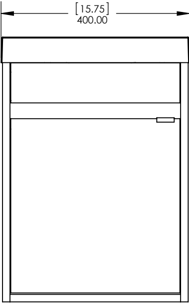
Front view / Vista Frontal
