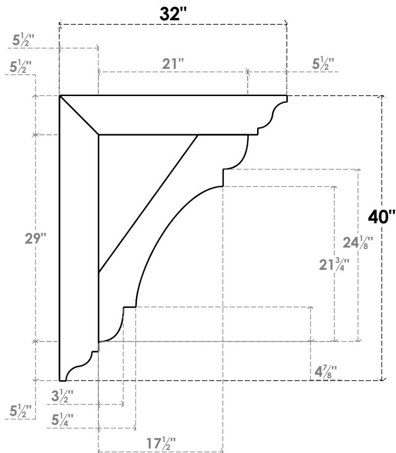
SIDE PROFILE
