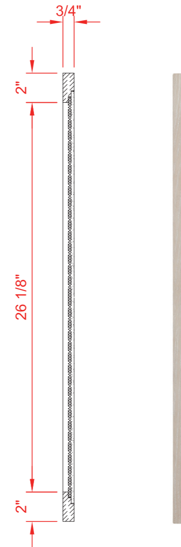
SIDE VIEW
