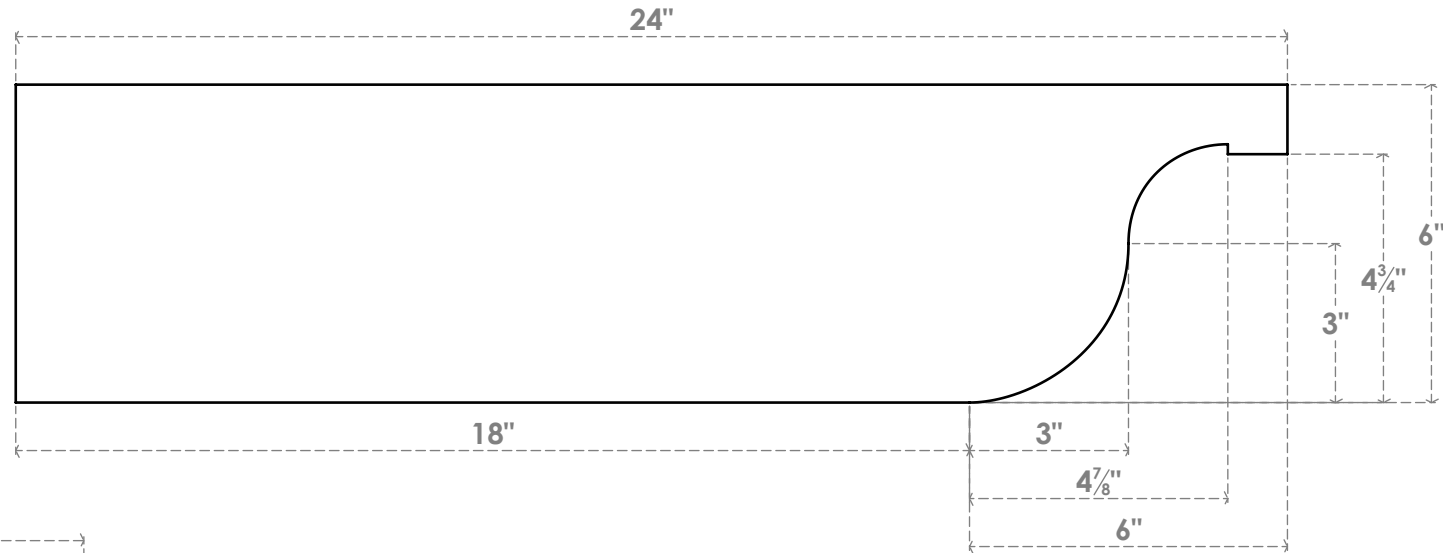
SIDE PROFILE
