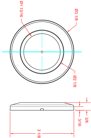
ICSS-CCR-COVER Detail
