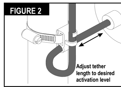
TETHERED SWITCH INSTALLATION
