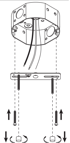
Mounting Screws
