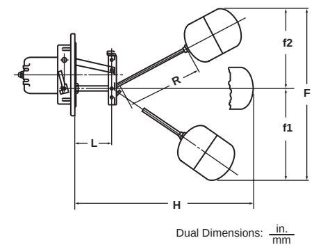
Figure 12: Float Position 3
