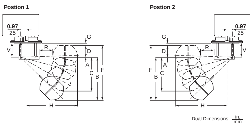
Figure 23: Travel Dimensions
