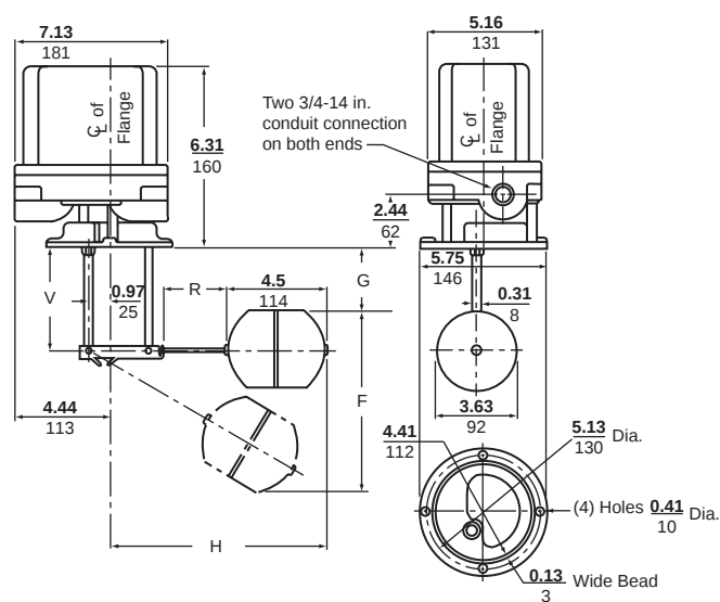
Figure 25: Type DR/DW Dimensions
