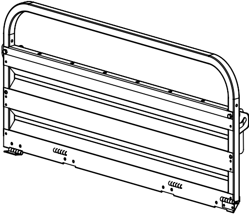
4' SHORT DELUXE FRONT/REAR GATE (504413) 5' SHORT DELUXE FRONT/REAR GATE (504414)
