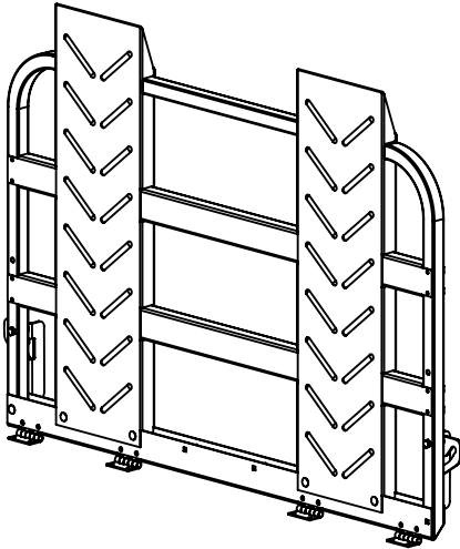
4' FULL REAR RAMP GATE KIT (504415)
