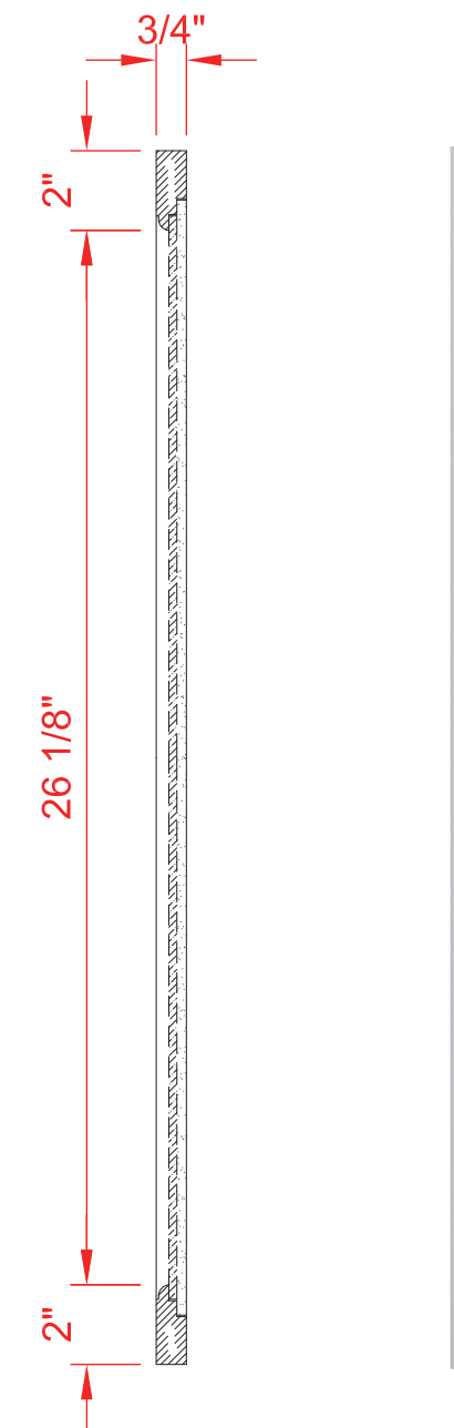
SIDE VIEW
