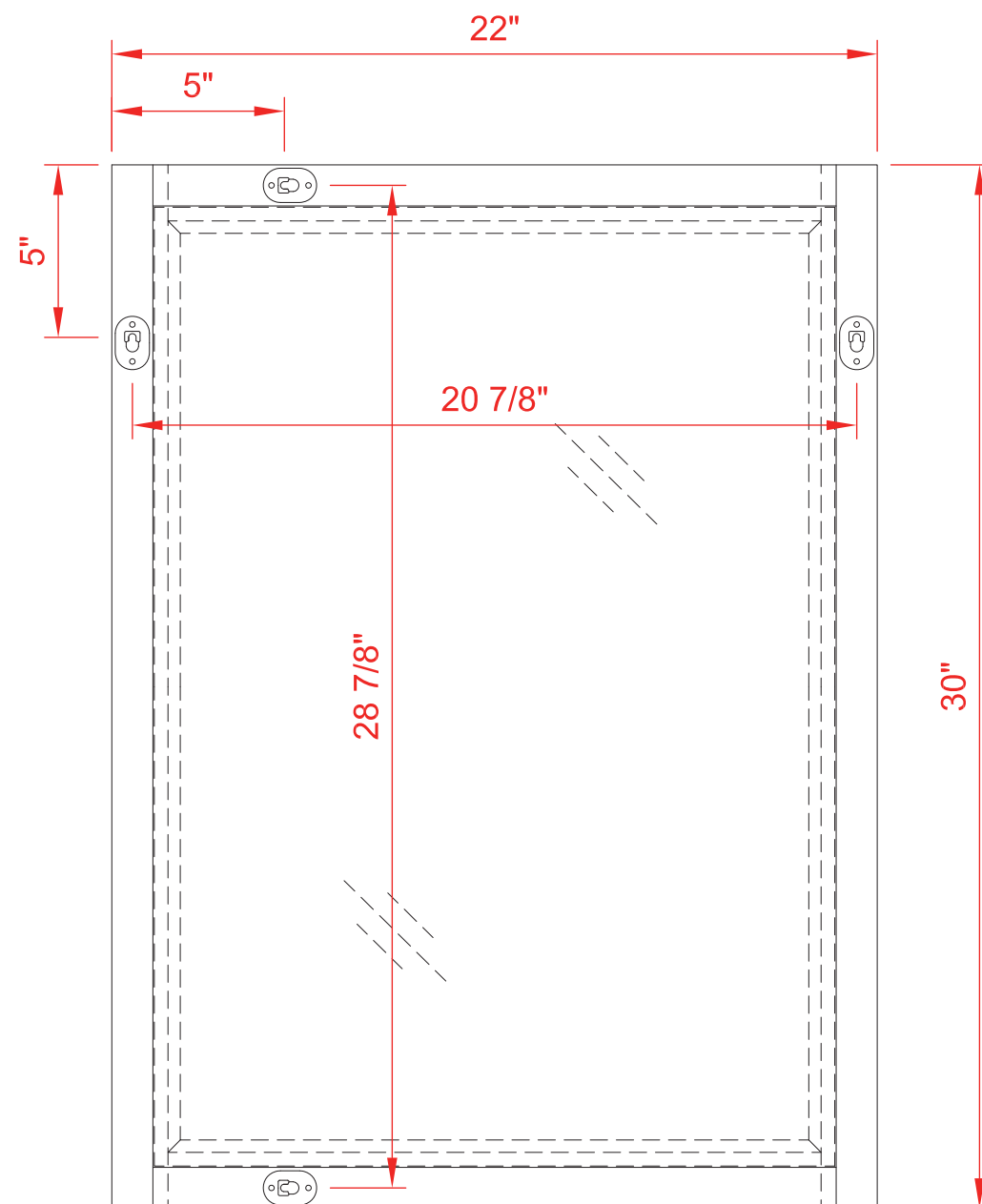
BACK VIEW
