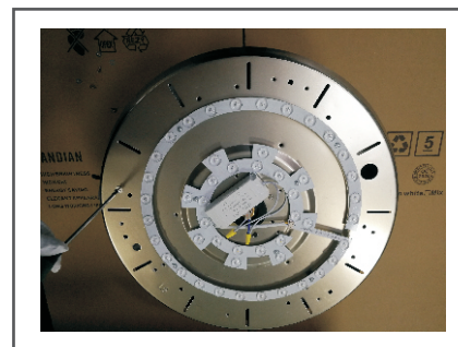
Step 4. Remove the main engine chassis screws.
