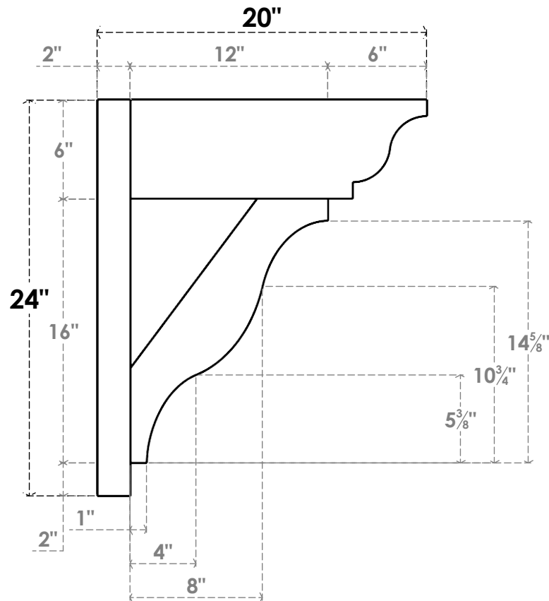
SIDE PROFILE
