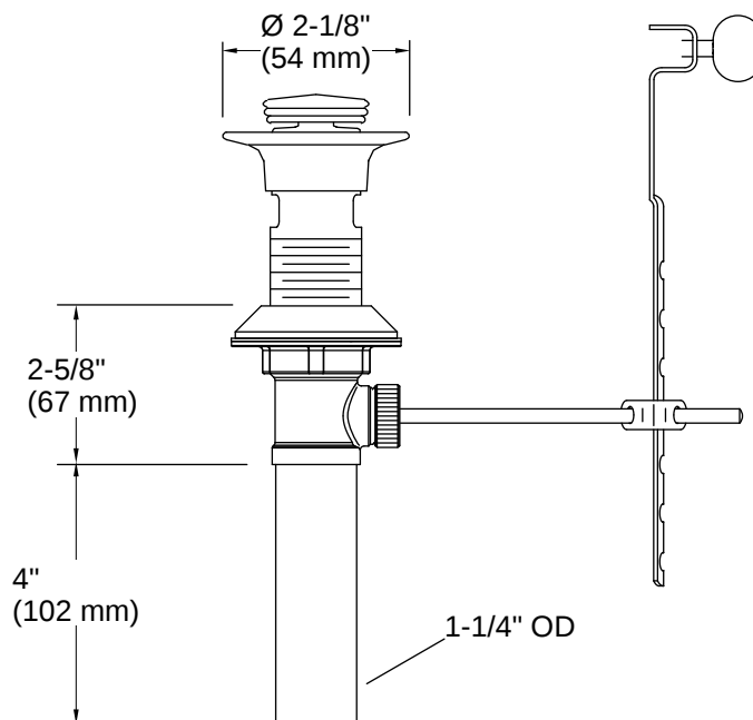
Pop-Up Drain
