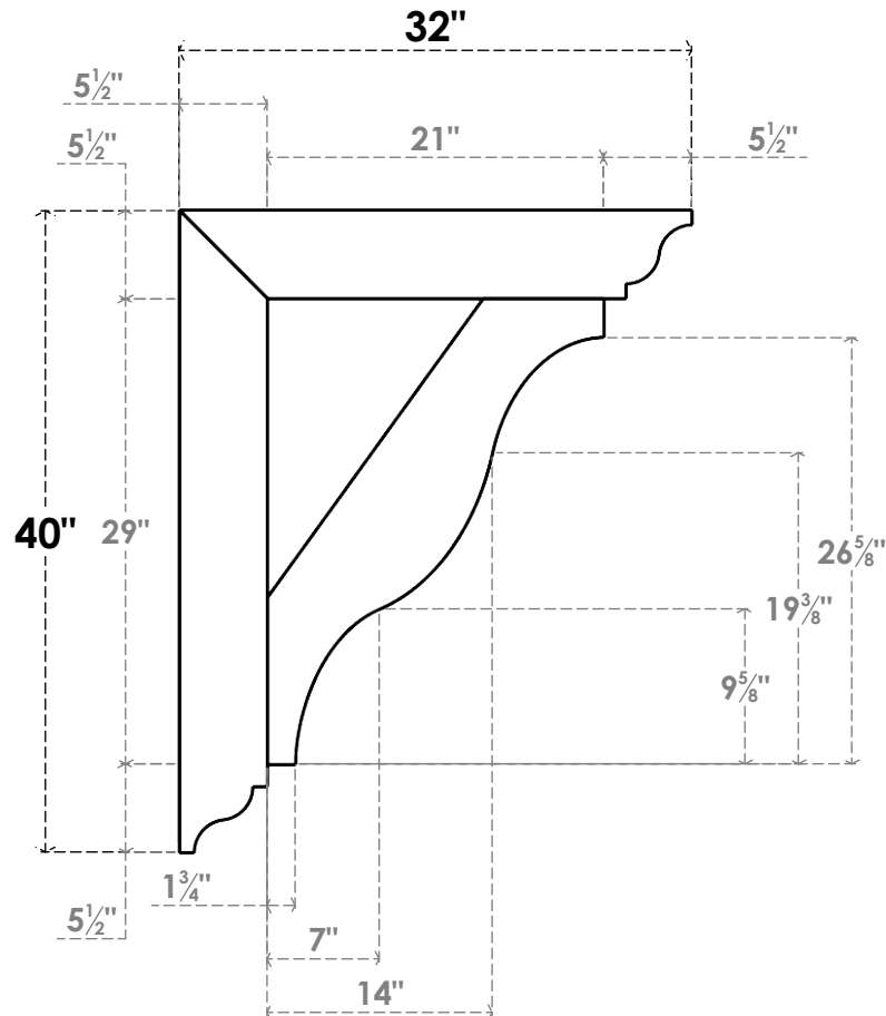
SIDE PROFILE
