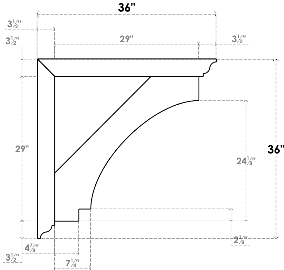
SIDE PROFILE
