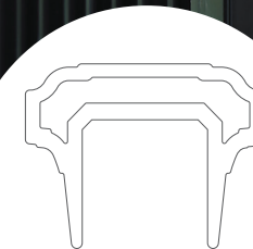
PREMIER RAILING® TOP RAIL SIZE: 3.5" X 2.7"
