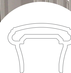
TRADEMARK RAIL™ TOP RAIL SIZE: 3.5" X 2.6" (ONLY AVAILABLE IN WHITE)
