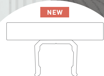
DRINK RAIL SELECT FROM ANY FULL PROFILE DECK BOARDS (NOT COMPATIBLE WITH GROOVED BOARDS)
