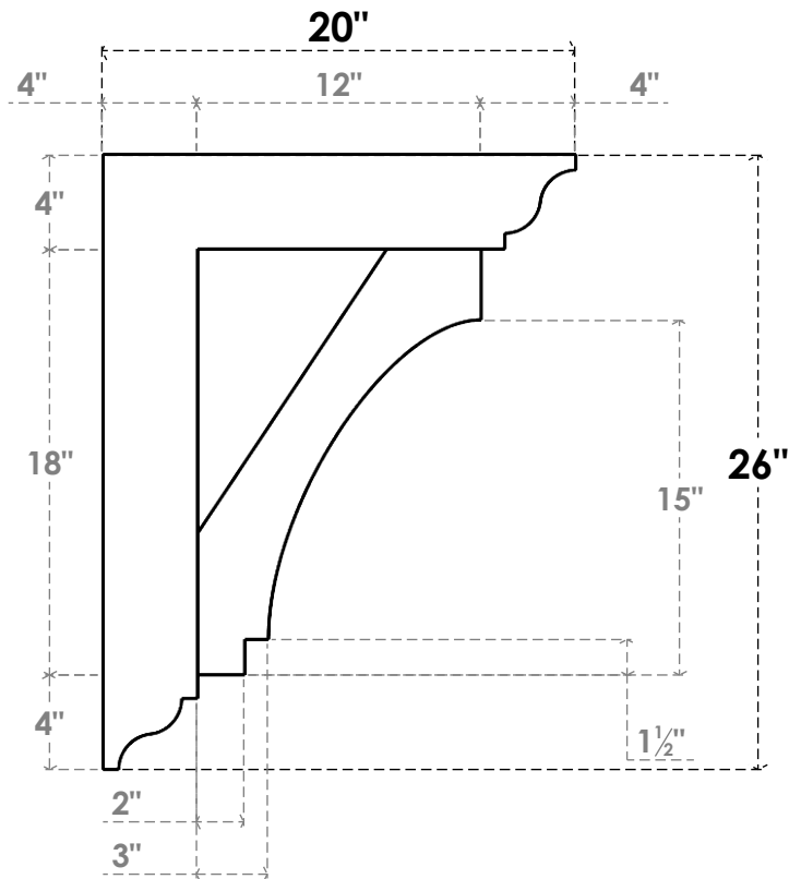
SIDE PROFILE
