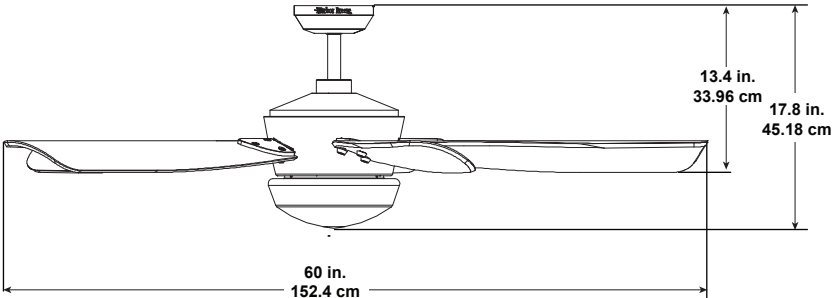
Downrod Standard
