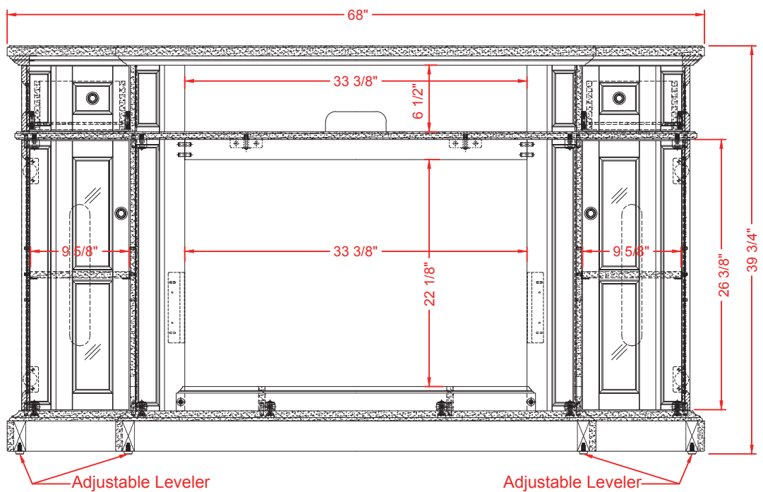
FRONT VIEW
