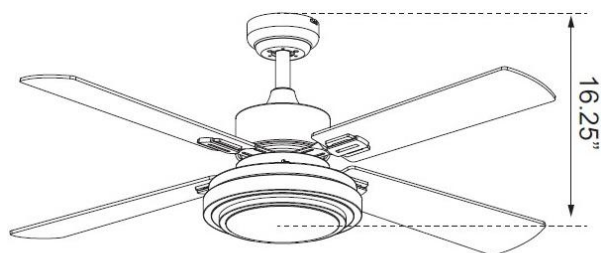
Total Height W/Downrod 16.25"
